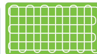
CRISS-CROSS APPLICATION
